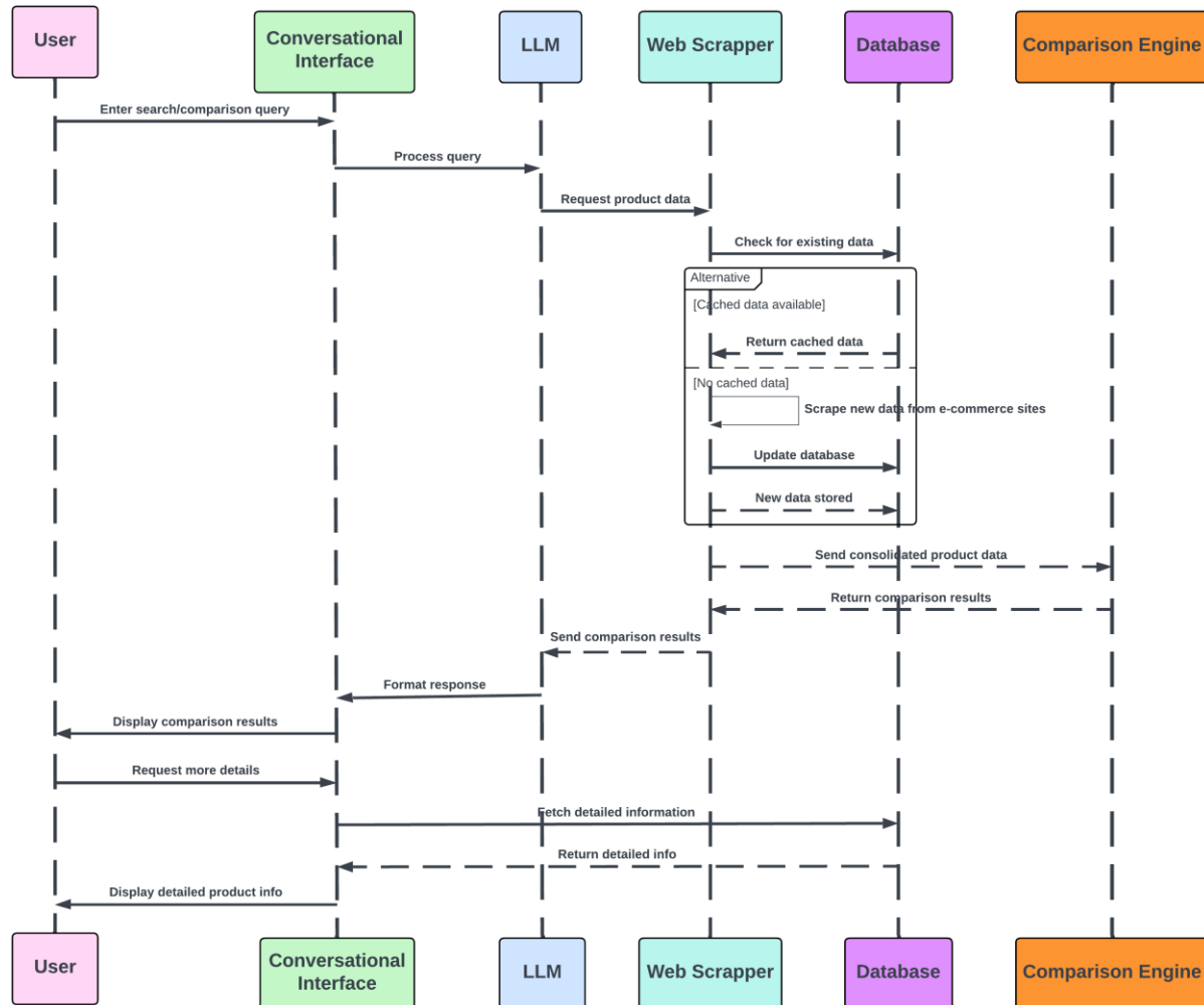
Figure 7 SSD use case 1
