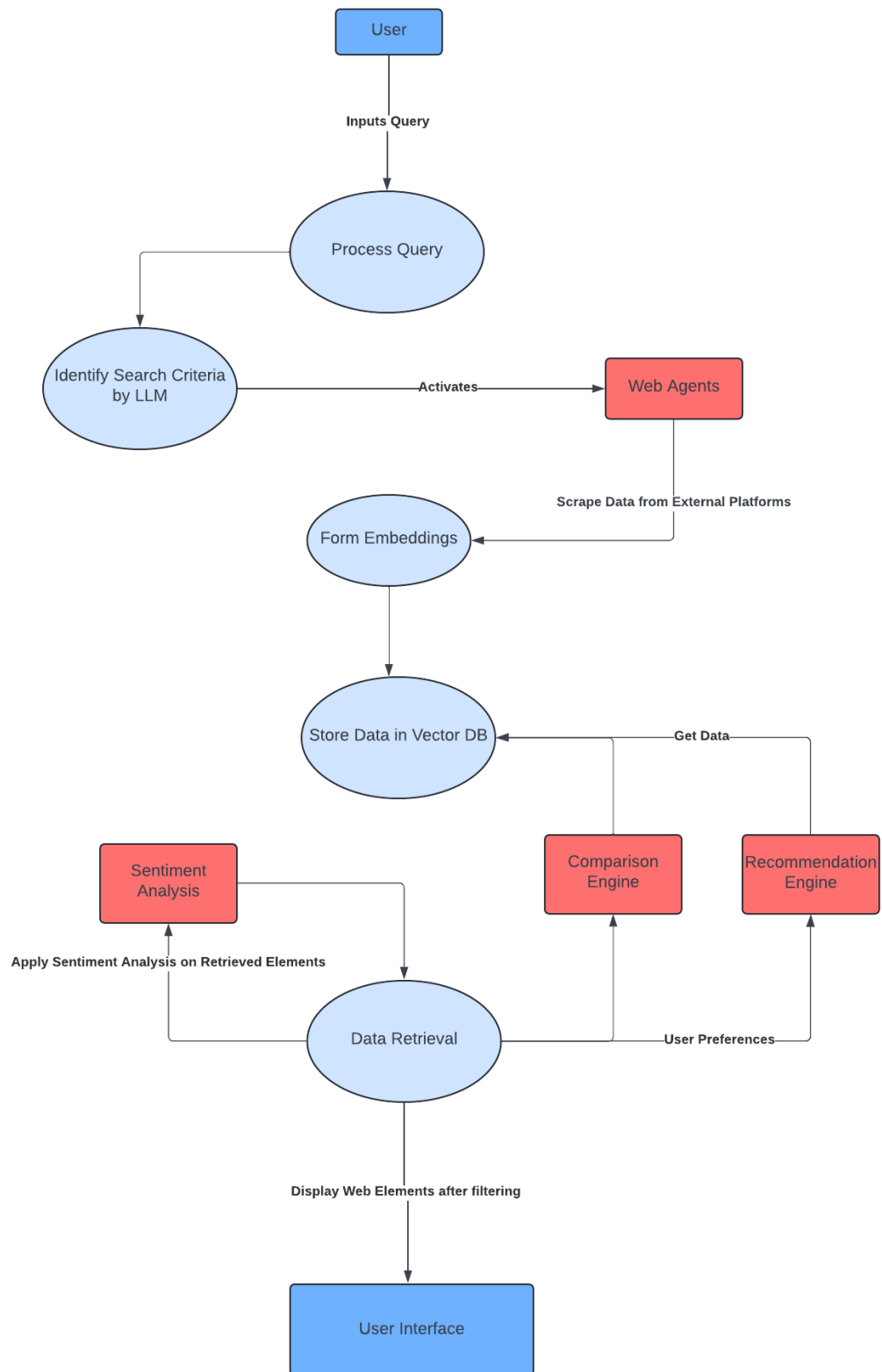
Figure 4 Data Flow Diagram Level 1
