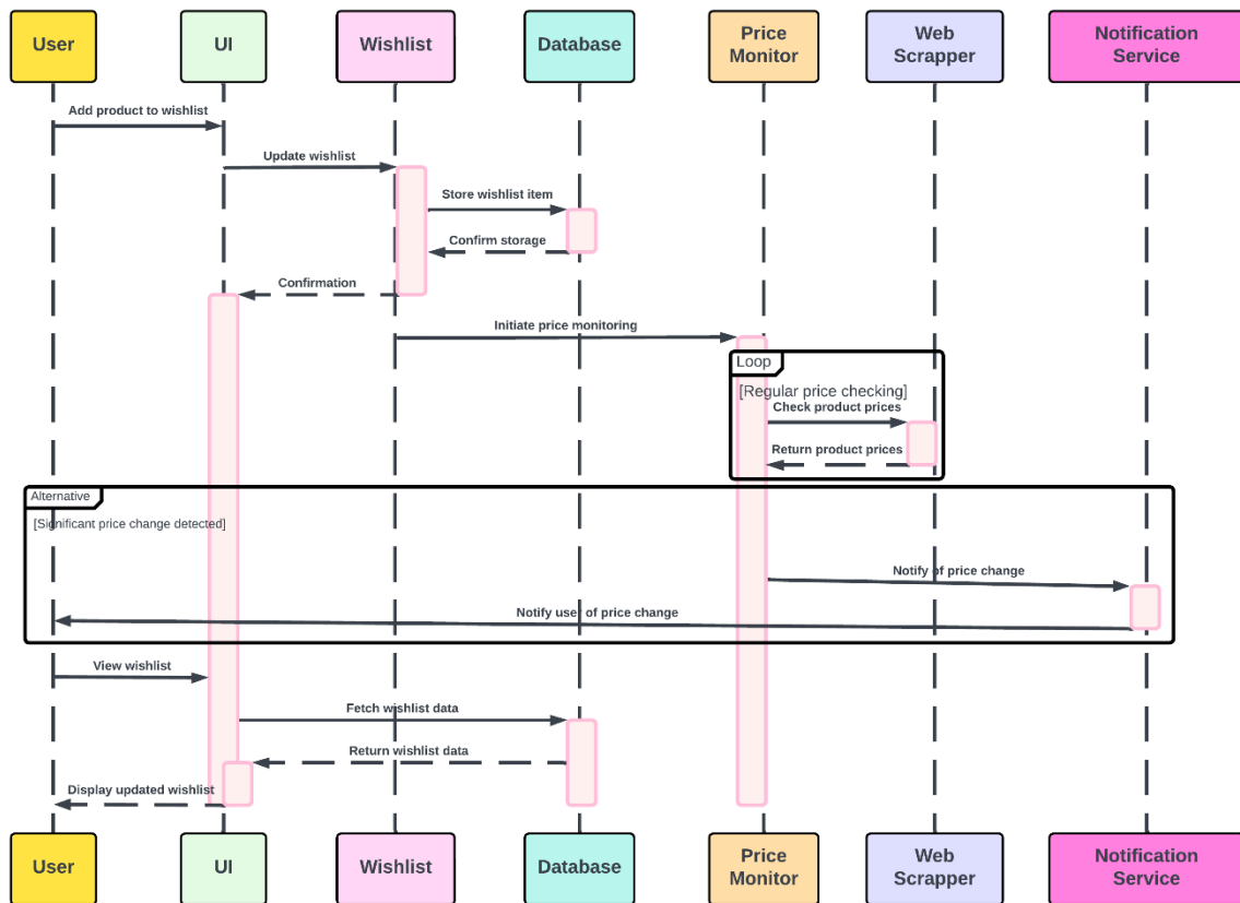
Figure 10 SSD use case 4
