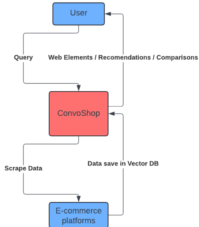
Figure 3 Data Flow Diagram Level 0
