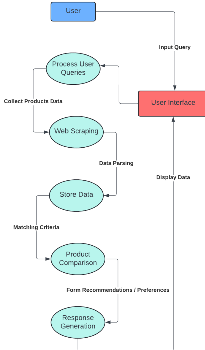
Figure 5 Data Flow Diagram Level 2
